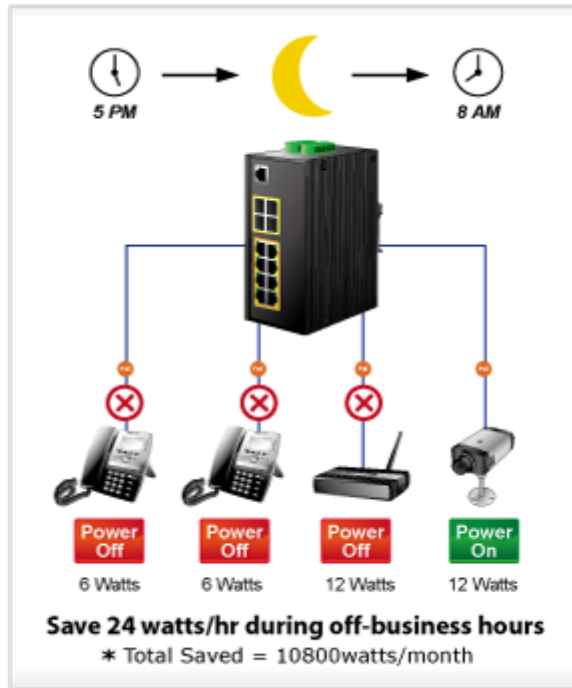
1000BASE-TX UTP with PoE
